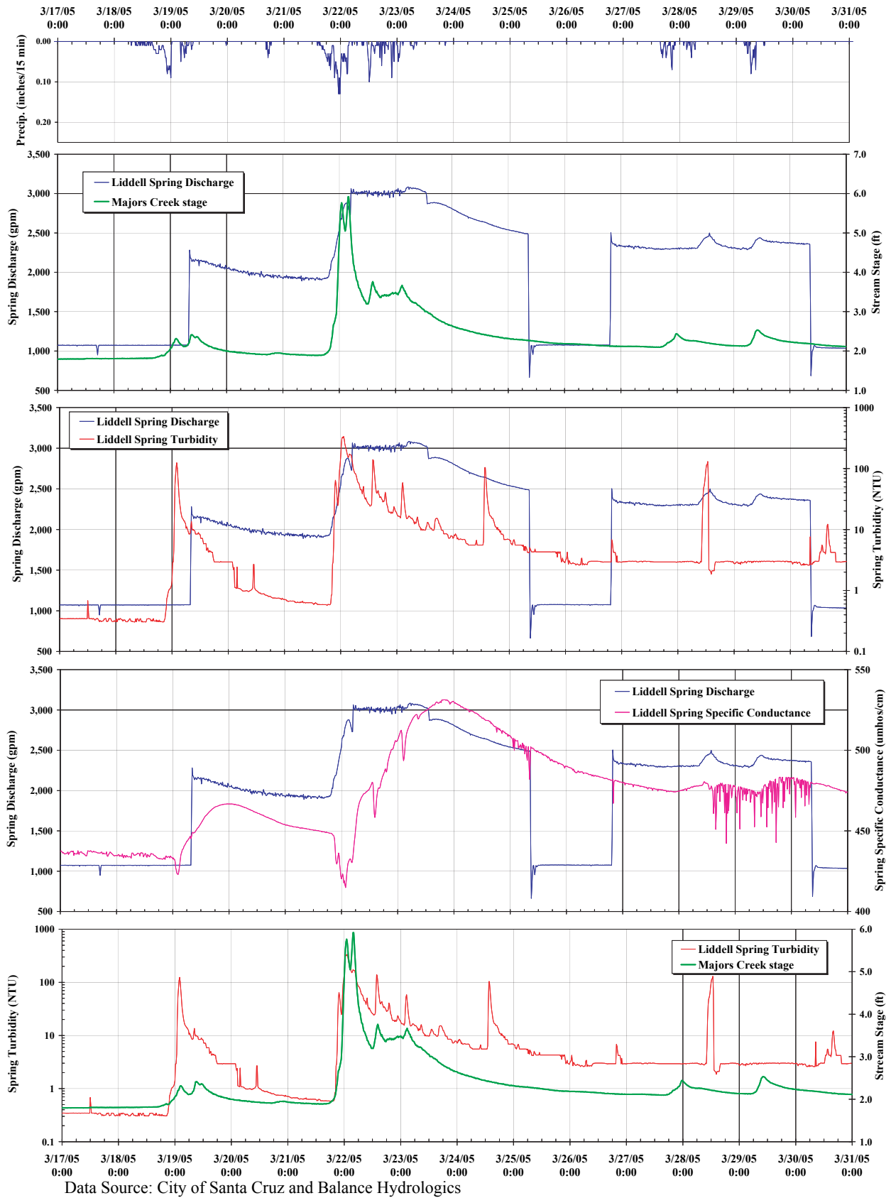
Storm Hydrograph Comparison, March 2005
